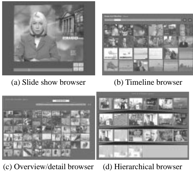
Fig. 3. Browsing interfaces
